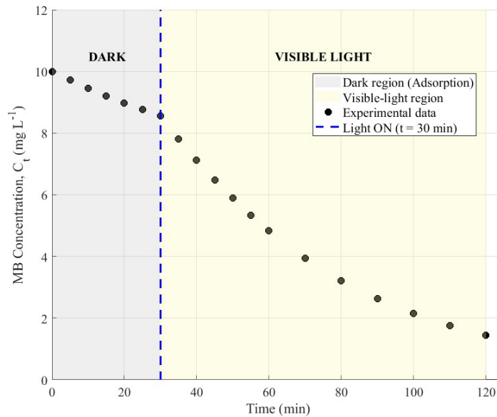
Fig. 4. Experimental concentration time profile of MB degradation. The dashed vertical line denotes the transition from dark adsorption to visible-light-driven photocatalysis
