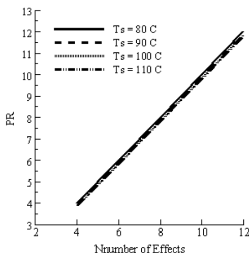
Fig. 4. Variation of the performance ratio as a function of the number of desalination effects for different feed water temperatures at a constant direct solar radiation intensity of 1000 W/m 2
