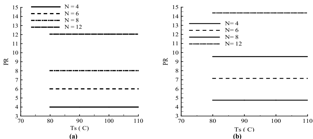
Fig. 5. The variation of performance ratio versus feed water temperatures at different desalination effect with (a) Q_{rad} = 0 W/m 2 and (b) Q_{rad} = 1000 W/m 2
