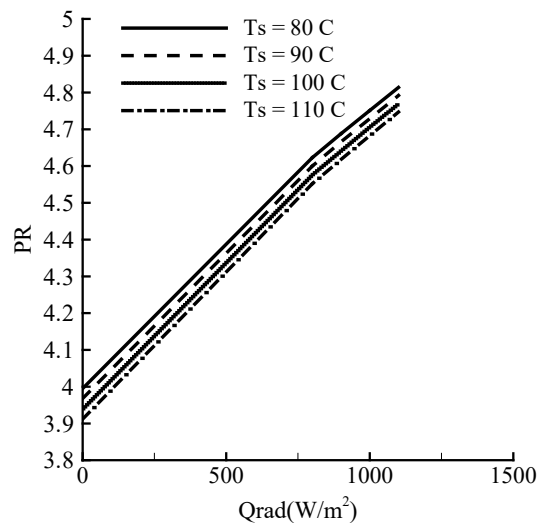
Fig. 6. The variation of performance ratio (PR) versus solar radiation on the different feed water temperatures for a fixed desalination effect of N=4
