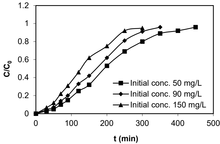
Fig. 4. Effect of inlet concentration on cobalt biosorption by Sargassum sp. (bed height 4 cm, feed flow rate: 1 mL/min)
