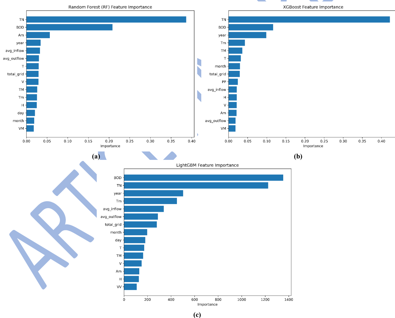
Fig. 3. Feature importance scores generated by (a) Random Forest (RF), (b) XGBoost, and (c) LightGBM using all 19 features
