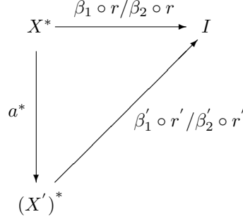
FIGURE 9. Commuting Diagram Equivalent to Diagrams in Figure 8
