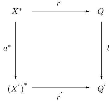
FIGURE 7. Commuting Diagram for Proposition 3.19
