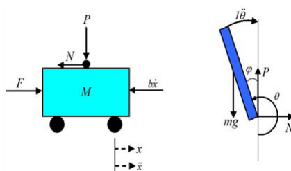
FIGURE 1. Pendulum system force analysis.
