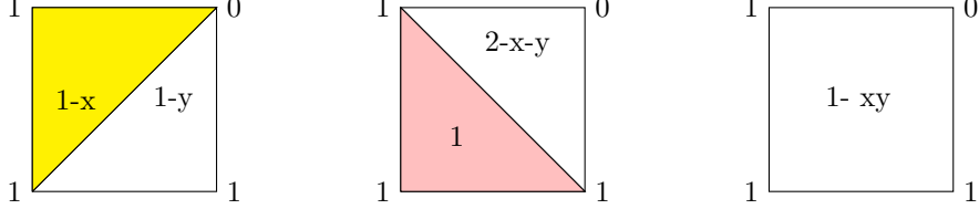
FIGURE 5. Linear Extensions of the Sheffer Stroke to [0, 1]^2
