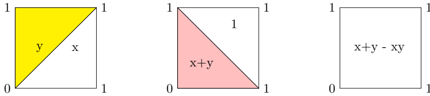
FIGURE 2. Linear Extensions of the Boolean Disjunction: Zadeh’s Disjunction (left); Łukasiewicz’s Disjunction (Middle); Probabilistic Sum (Right)
