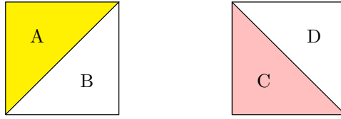
FIGURE 1. Simplexes for Linear Extensions of Binary Boolean Functions
