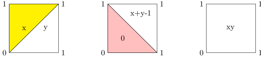
FIGURE 3. Linear Extensions of the Boolean Conjunction: Zadeh’s Conjunction (Left); Łukasiewicz’s Conjunction (Middle); Product (Right)
