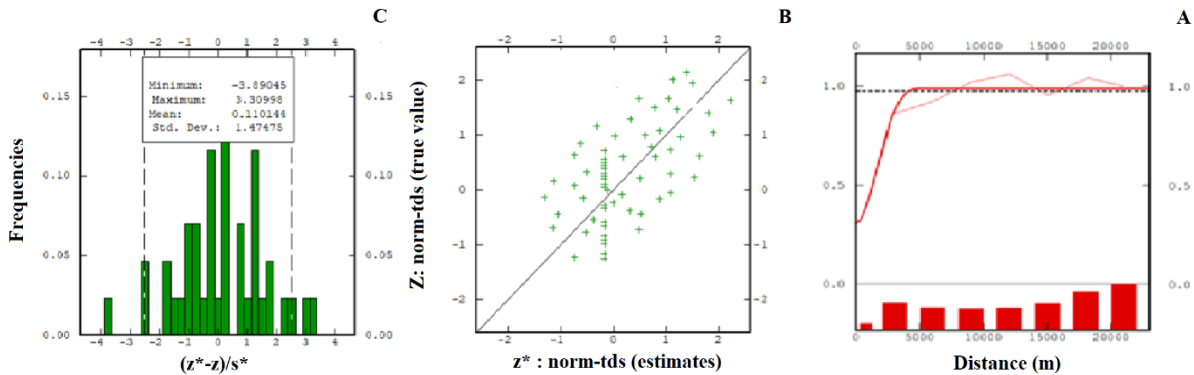
Fig. 4. A) Variogram diagram of the average values of arsenic. B) Correlation diagram. C) Remaining values histogram.
