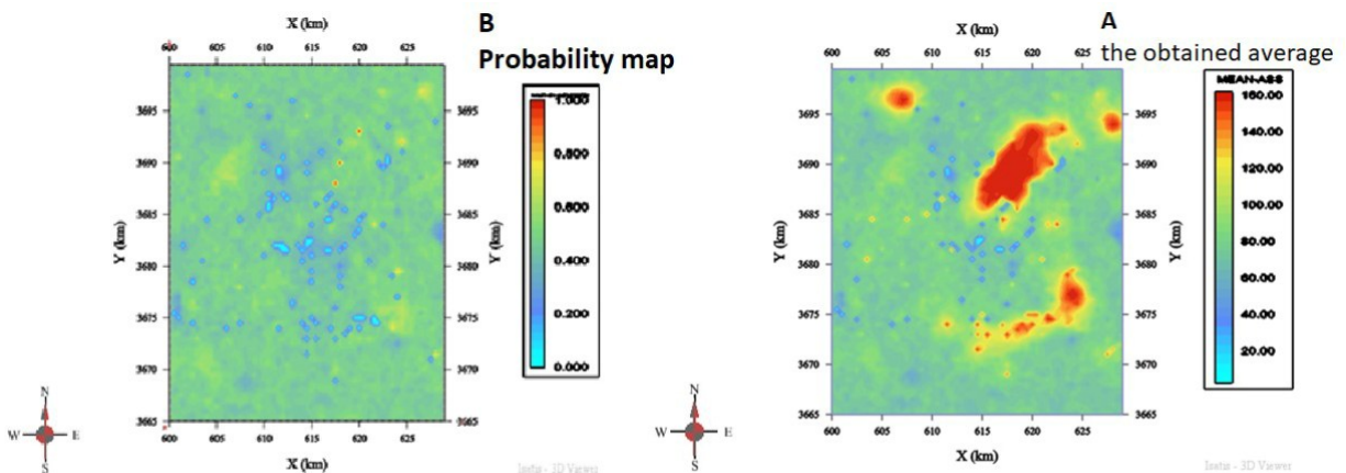
Fig. 7. A) The obtained average from the Gaussian simulation B) Diagram of the uncertainty of the arsenic above the allowable value.
