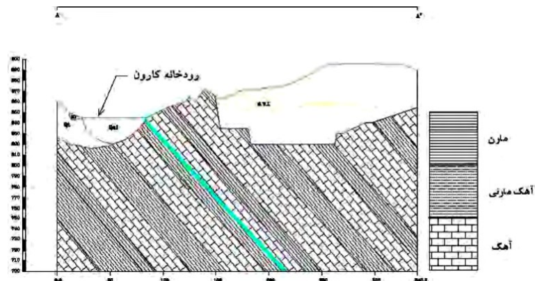
Fig. 3. Cross-section AA' with a depth of 120 meters of the impervious boundary of the bottom from the water level in the Karun River.
