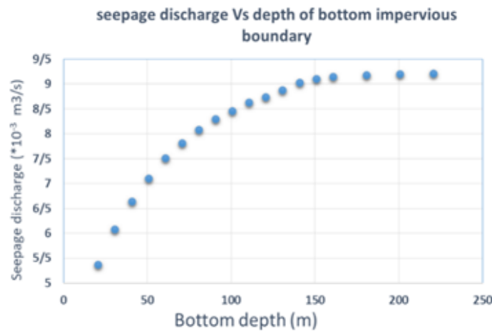
Fig. 4. Seepage discharge according to the depth of bottom impervious boundary.
