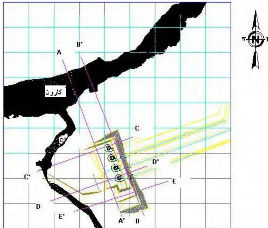
Fig. 2. Location of power plant trench and five sections of seepage analysis.
