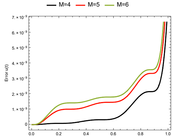
Fig. 1. Absolute errors with k = 1, \beta(t) = 1 for Example 1.
