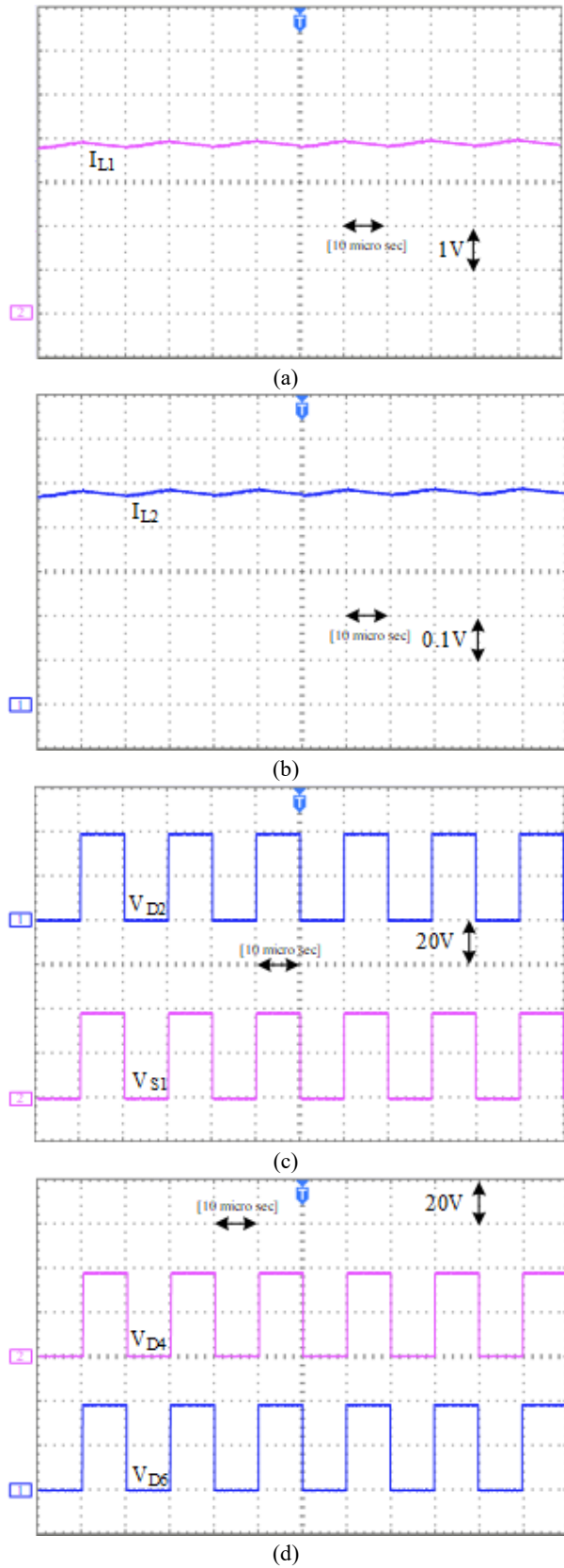
Fig. 15. Experimental results of the proposed converter. (a) I_{L1} , (b) I_{L2} , (c) V_{S1} , V_{D2} , and (d) V_{D4} , V_{D6} .
