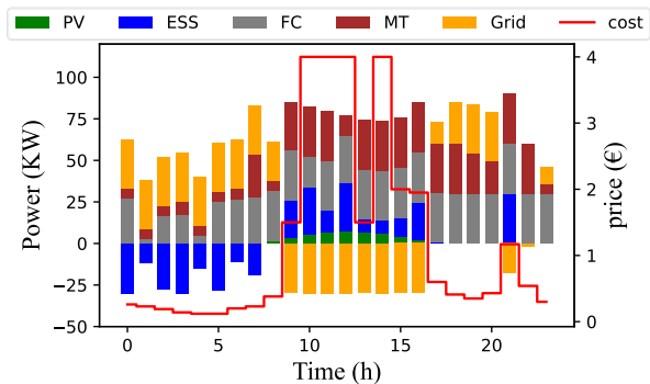
Fig. 5. QIO results for Scenario 2.
