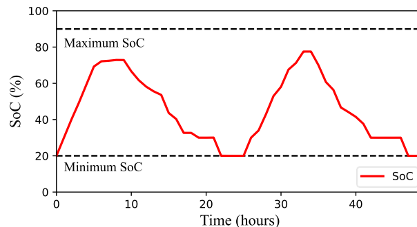
Fig. 6. SoC profile of test days.
