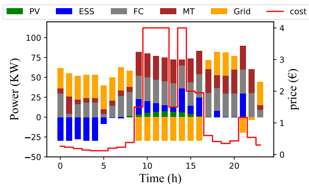
Fig. 4. QIO results for Scenario 1.
