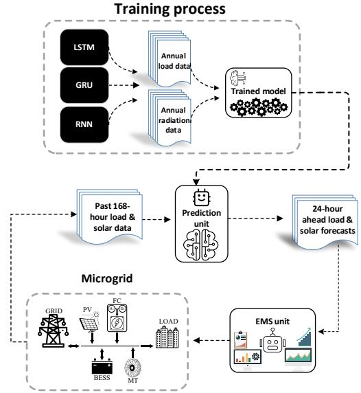
Fig. 2. Schematic of the predictive control methodology.
