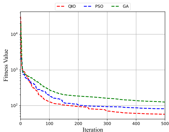
Fig. 7. Convergence curves of the algorithms for Scenario 1.
