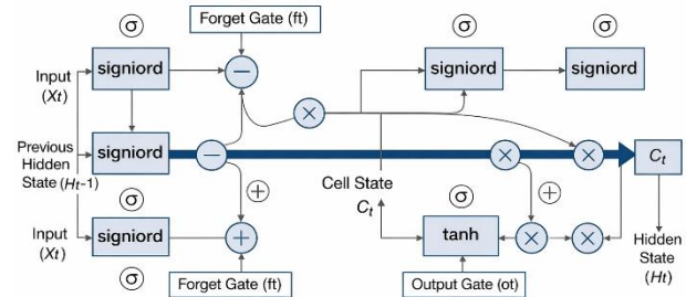
Fig. 1 LSTM model
