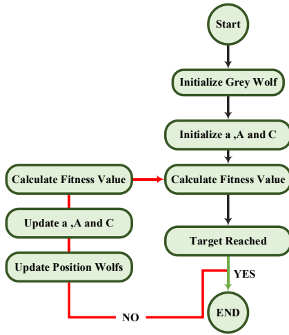
Fig. 4. Flowchart of the GWOA.
