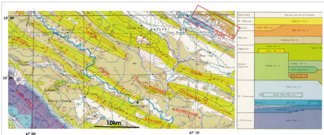
Fig 3: The geologic map of the study area (part of the Ilam-Kuhdasht 1:250,000 geologic map, Llewellyn 1974), the Amiran Formation has been highlighted by a frame.
