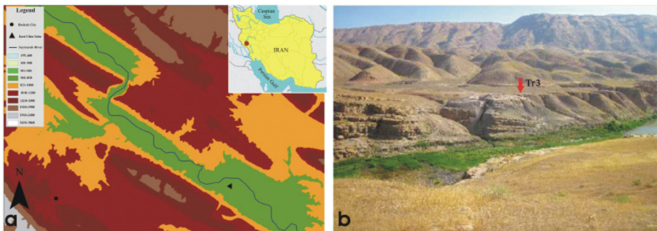
Fig 1: a) Location of the East Chia Sabz and part of the Seymareh River; b) an overview of the East Chia Sabz at the Seymareh River, looking to the south (pictures modified after MirBolouki et al. 2015).
