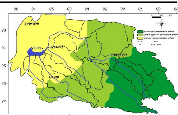
Fig 5. Precipitation zones of Helmand basin
