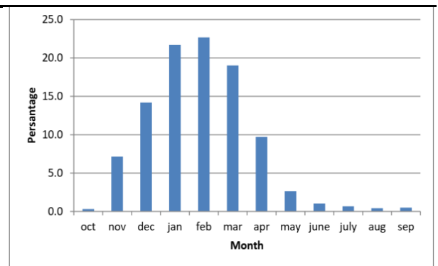
Fig 8. The pattern of monthly relative rainfall of precipitation regime of Helmand basin
