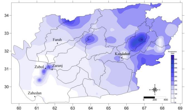
Fig 2. The spatial distribution of mean annual rainfall in Helmand basin by using TRMM satellite data for the period of 2000-2014
