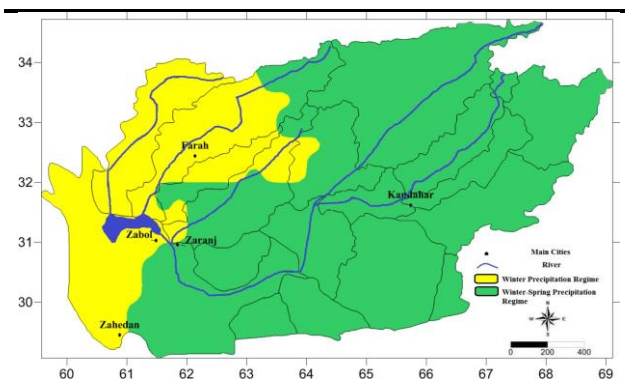
Fig 7. Zoning of precipitation regimes by using points taken from TRMM satellite for Helmand basin
