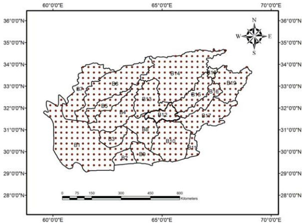
Fig 3. Number and geographical positions of monthly precipitation points taken from TRMM satellite
