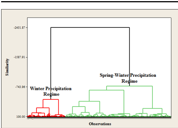
Fig 6. Dendrogram resulted from cluster analysis on monthly relative precipitations of points taken from TRMM satellite for Helmand basin
