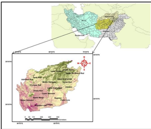
Fig 1. Geographical location of Helmand basin in South West Asia
