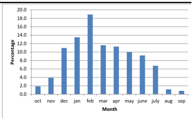
Fig 9. Monthly relative rainfall pattern of winter-spring precipitation regime Helmand basin
