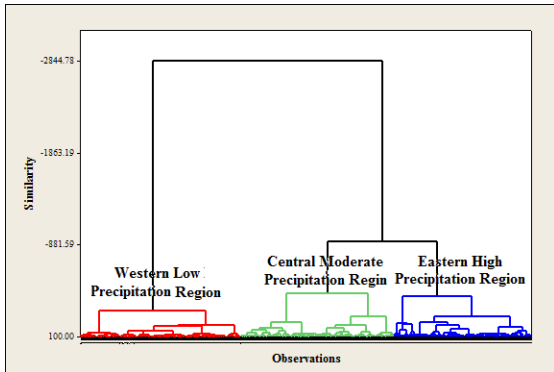
Fig 4. Dendrogram resulting from cluster analysis on the matrix of annual rainfalls of Helmand basin
